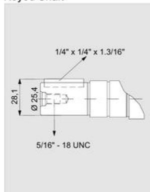
Keyed Shaft
