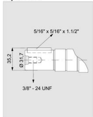
Keyed Shaft
